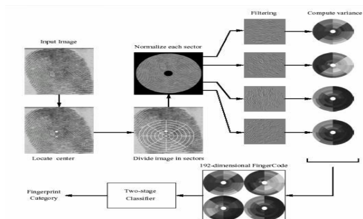
Fig 5: Classification of finger print from input image/fingerprint.
