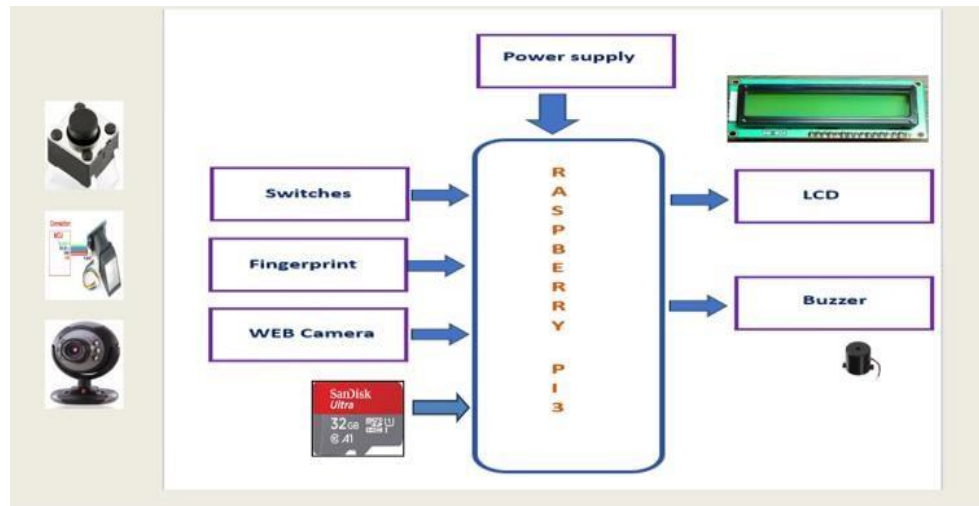
Fig 6. Block Diagram of System.
